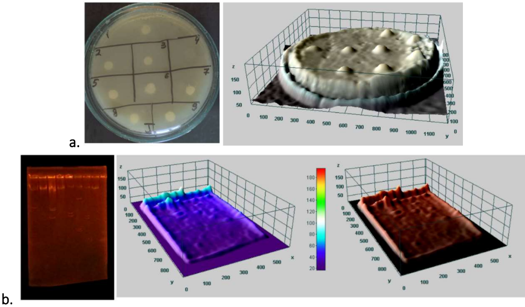
Fig. 1. A: Resistance tests of B. laterosporus 194-1, L. sphaericus 2626, L. sphaericus 288 on solid cultural media and the digital analysis of it; B: DNA Electrophoresis of B. laterosporus 194-1, L. sphaericus 2626, L. sphaericus 2884 and digital analysis of it.
